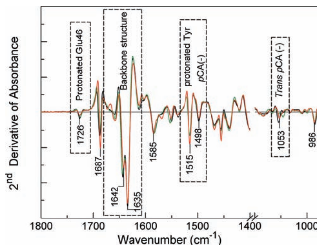
Figure 5. Probing structural deformations of the pG dark state of wtPYP (black) by the N43A (red) and N43S (green) mutations using second derivative FTIR spectroscopy. The FTIR absorbance spectrum of the three protein samples was measured at 2 cm^{-1} resolution and was used to calculate the second derivative to facilitate comparison of spectral features in the three spectra. Selected peak positions are indicated.
