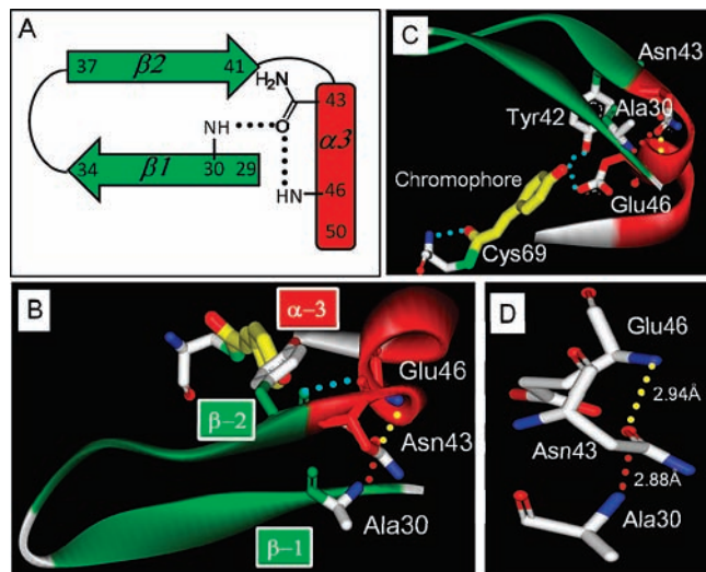
Figure 2. Side-chain hydrogen bonding of Asn43 in PYP. (A) Cartoon of the conserved hydrogen-bonding pattern (residue numbering for PYP). (B and C) Residues 28–50 of PYP (1NWZ) shown in two orientations, together with the pCA . Selected hydrogen bonds are shown as dotted lines, \alpha -helices are shown in red, and \beta -strands are in green. The helical capping hydrogen bond is shown in yellow, while the structural bridging hydrogen bond is in red. (D) Zoom-in to highlight the hydrogen-bonding interactions of Asn43.
