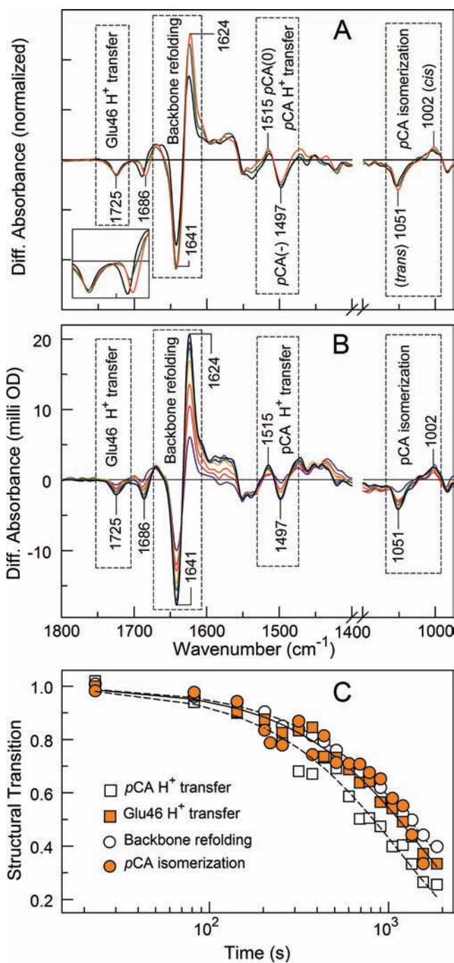
Figure 7. Structural changes upon pB formation in wtPYP and its N43A and N43S mutants detected by FTIR difference spectroscopy. (A) The pB – pG infrared difference spectra at 4\text{ cm}^{-1} resolution for wt (black), N43A (red), and N43S (green) PYP ( \text{pH}^* = 6.6 ) were derived from flash-induced time-resolved rapid scan FTIR spectra. The inset shows a magnification of the peaks near 1726 and 1689\text{ cm}^{-1} . (B) Time-resolved FTIR difference spectroscopy during pB decay in N43A PYP. The plotted spectra range from 8 to 1712 s. The region 1100\text{--}1400\text{ cm}^{-1} is not shown because it does not contain relevant vibrational marker signals. (C) Amplitude-normalized kinetics of structural events during pB decay in N43A PYP. The data from (B) were used to extract the kinetics of Glu46 protonation ( 1725\text{ cm}^{-1} ), pCA deprotonation ( 1515 and 1497\text{ cm}^{-1} ), pCA reisomerization ( 1051\text{ cm}^{-1} ), and backbone conformational changes ( 1641 and 1624\text{ cm}^{-1} ). The transitions were fitted as monoexponential decays (lines), yielding lifetimes of 1640, 1190, 1630, and 1880 s (see main text).
