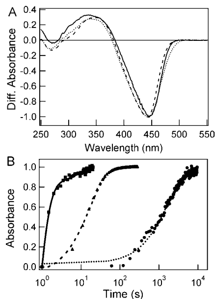
Figure 6. Substitutions at Asn43 slow the kinetics of the last PYP photocycle step. The pB – pG UV/vis absorbance difference spectra (A) and kinetics of the pB to pG transition (B) for wtPYP (solid lines and ■), N43S PYP (dashed lines and ▲), and N43A PYP (dotted lines and ●) at pH 7.1 are shown. The difference spectra were normalized for the extent of bleaching of the pG state. The kinetics of the wtPYP photocycle were fitted as a biexponential decay, while those of N43A and N43S PYP were fitted as a monoexponential decay. The amplitudes of the kinetic traces were normalized; the optical densities of the samples at their visible absorbance maxima near 445 nm were in the 0.35–0.45 range.
