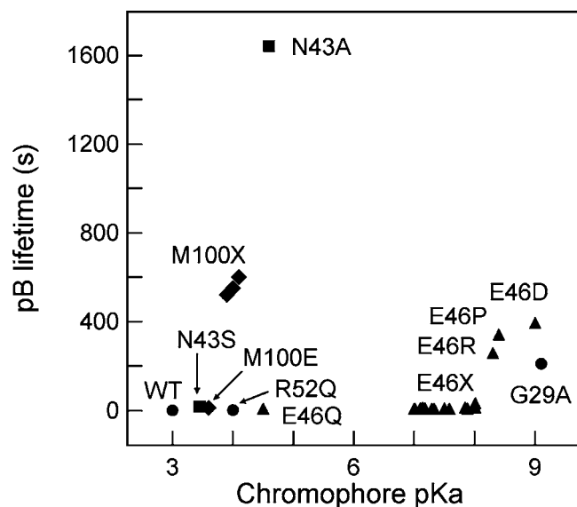
Figure 8. Comparison of functional properties of PYP mutants. The pK_a of the pCA in the pG state and the lifetime of the pB state for all mutants for which both of these properties have been reported are depicted. Substitution mutants at position Asn43 are indicated as ■, those at Glu46 as ▲, and at Met100 as ◆; the remaining proteins are depicted by ●. The cluster of mutants indicated as M100X consists of the A, L, and K substitution mutants of Met100; cluster E46X contains the A, C, G, H, I, K, L, N, S, T, V, W, and Y substitutions of Glu46.
