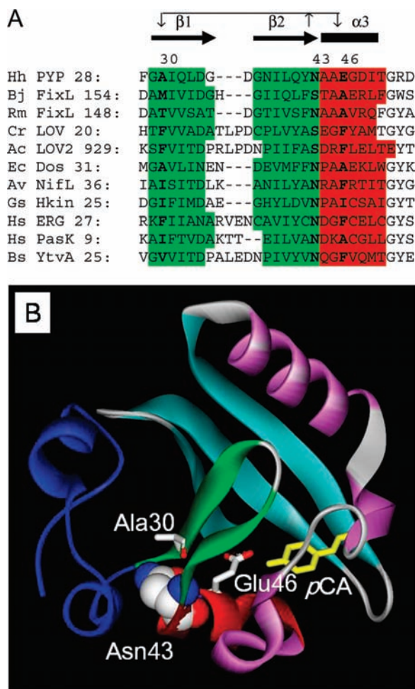
Figure 1. Sequence conservation and structural context of Asn43 in PYP. (A) Multiple sequence alignment of the N-terminal region of PAS domains with conserved side-chain hydrogen bonding at residue 43. The PAS domain residue numbering used here is based on the PYP from Halorhodospira halophila . The number of the first depicted residue of each PAS domain is shown. The sequence alignment was adjusted on the basis of the known three-dimensional structure of these PAS domains. Secondary structure is indicated: \alpha -helices are shown in red and by the thick black bars; \beta -strands are indicated in green and by the black arrows. Residue 43 and its two key hydrogen-bonding partners in \beta -strand 1 and \alpha -helix 3 are highlighted in bold. The conserved side-chain hydrogen bonds of residue 43 with the backbone amide groups of these two residues are indicated by arrows. Hh = Halorhodospira halophila ; Bj = Bradyrhizobium japonicum ; Rm = Rhizobium meliloti ; Cr = Chlamydomonas reinhardtii ; Ac = Adiantum capillus-veneris ; Ec = Escherichia coli ; Av = Azotobacter vinelandii ; Gs = Geobacter sulfurreducens ; Hs = Homo sapiens ; Bs = Bacillus subtilis . (B) Schematic representation of the crystal structure of PYP highlighting Asn43. The side chain of Asn43 is shown in CPK coloring. As in panel (A), \alpha -helix 3 is shown in red, while \beta -strands 1 and 2 are indicated in green. The pCA chromophore is depicted in yellow, and the N-terminal region of PYP is in dark blue.
